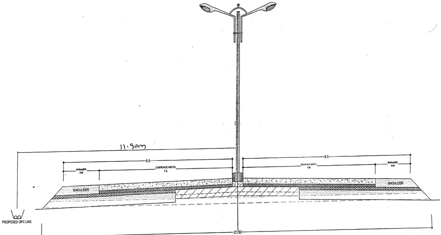
TYPICAL CROSS SECTION e km. 112.338 4 - LANE DIVIDED CARRIAGEWAY
