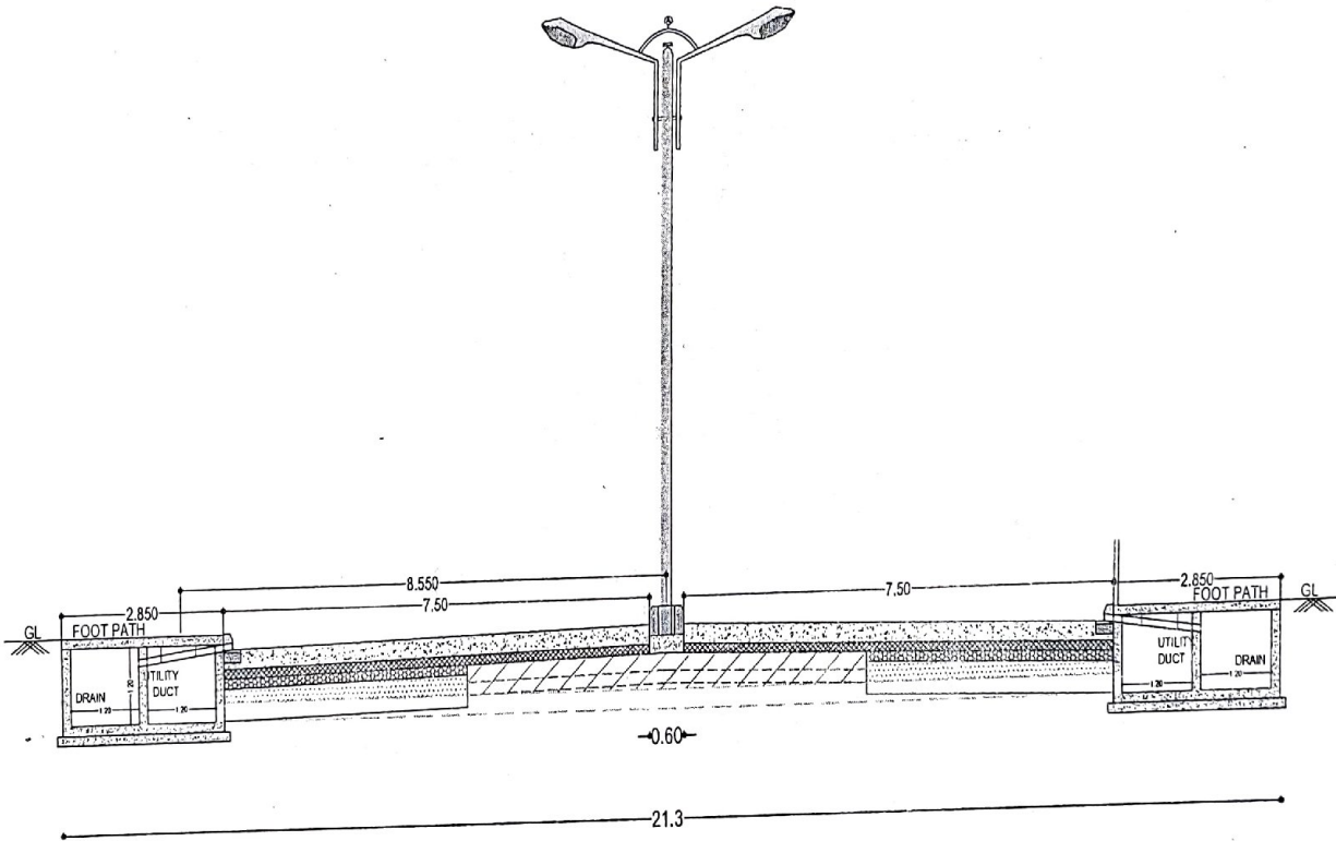
TYPICAL CROSS SECTION @ KM-107.500
