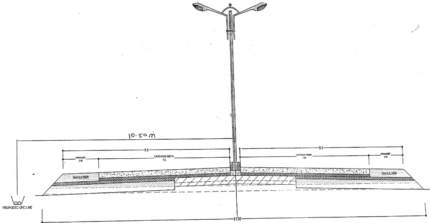
TYPICAL CROSS SECTION @ Km. 111.450
