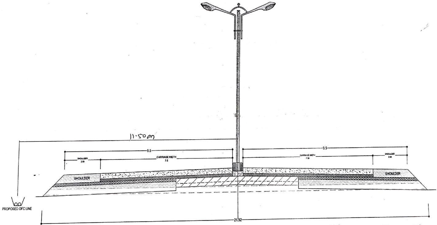
TYPICAL CROSS SECTION @ km. 110.442 4 - LANE DIVIDED CARRIAGEWAY
