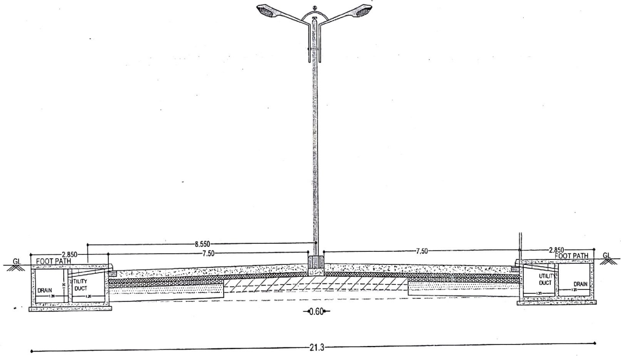
TYPICAL CROSS SECTION @ KM- 108.500
